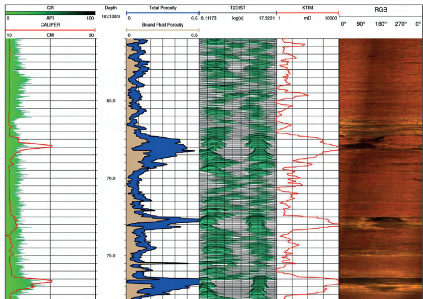
Hydraulic conductivity driven by vugs and fractures
