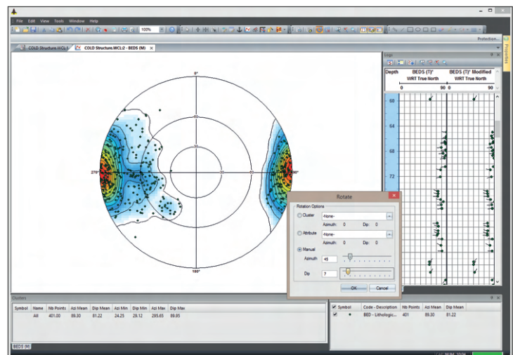
Dips Workspace
