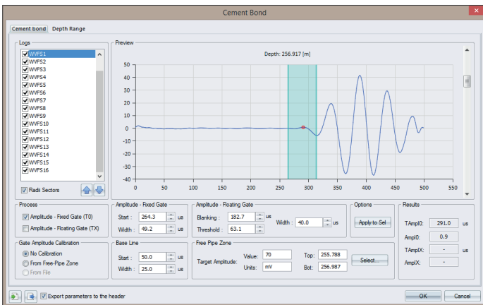
Cement Bond Processing for CBL and RBT tools
