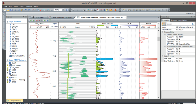
NMR workspace
